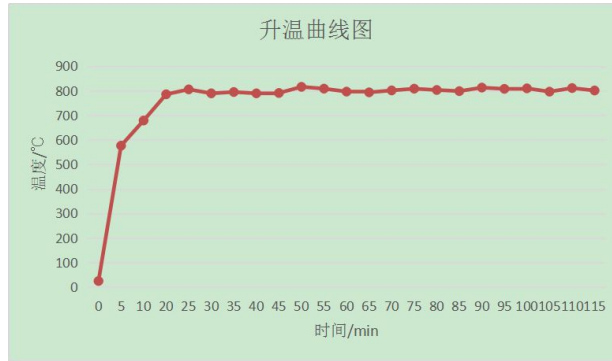
耐火试验-时间温度曲线图 Fire resistance test-Time temperature curve
